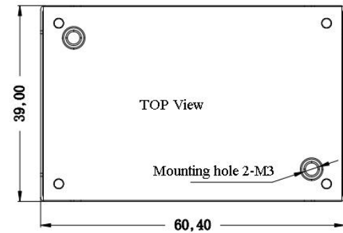
Standard 60.4*39.0*12.7mm
